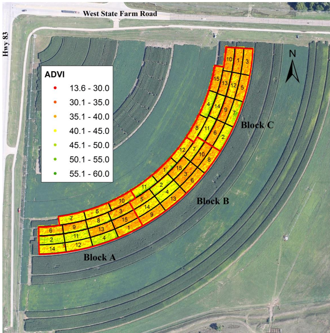
Figure 1. Airscout ADVI image collected on 8/11/17 by Ag Valley Coop for the 2017 UNL-TAPS Farm Management Competition held at the West Central Research and extension Center in North Platte, NE. The Farm ID's (i.e., treatments) are identified in the figure.
